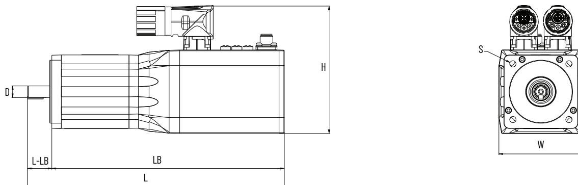
DSM Module Dimensions Table, 75 mm Frame Size
