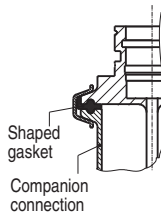
Figure 3 Mounting instructions for installation in hygienic processes
