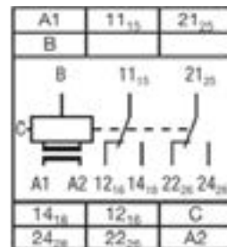
CM-ESS.M
