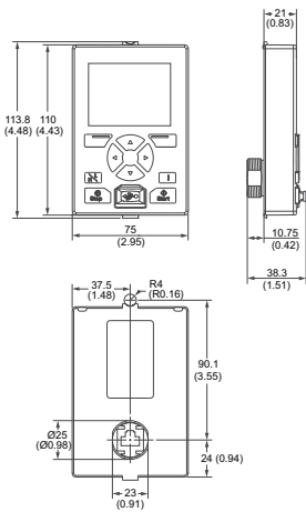
PSTX panel desmontable
