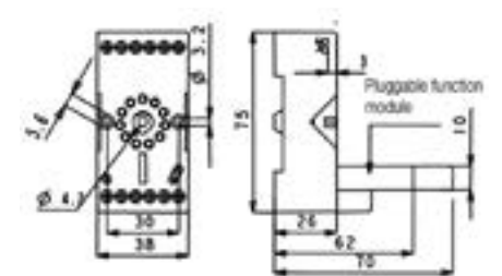
Base CR-U3S
