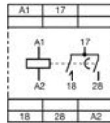
CT-SDS.22
