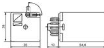
Relevador CR-U 3 C/O (11 pines)
