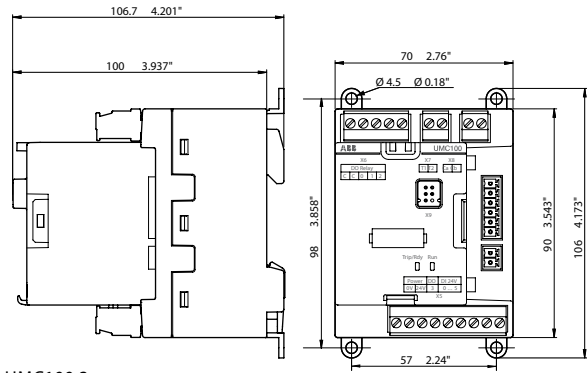
UMC100.3
