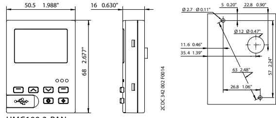
UMC100.3-PAN
