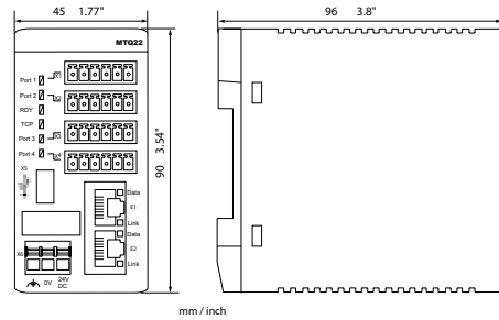
PNQ22, MTQ22
