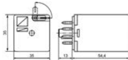
Relevador CR-U 2 C/O (8 pines)
