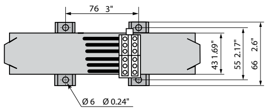
CT4L185R/4, CT4L310R/4
