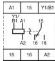
CT-ERD.13
