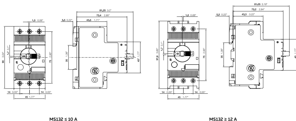
MS132 ≤ 10 A
