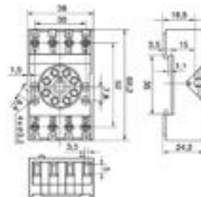
Base CR-U2SM
