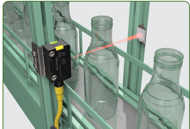
Clear object detection – clear objects such as bottles are difficult for standard sensors to detect because they see through the target. The 42JT clear object sensor reliably detects these objects thanks to specialized optics.
