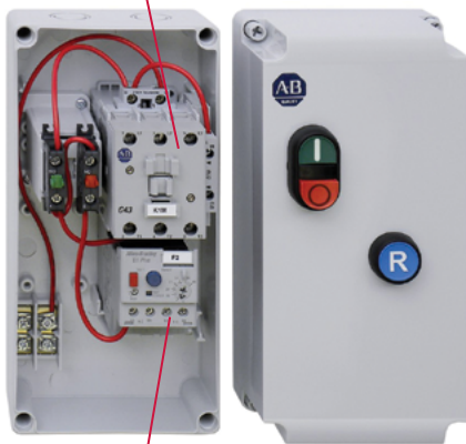
E1 Plus Electronic Overload Relay
