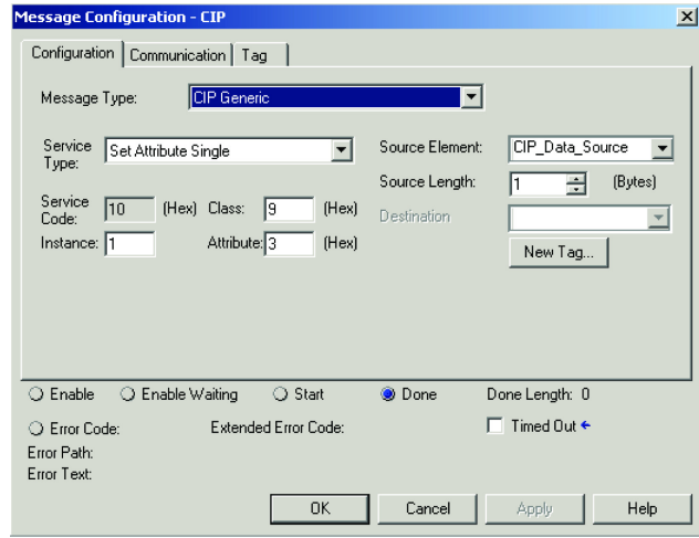
Figure 37 - Set State of Output
