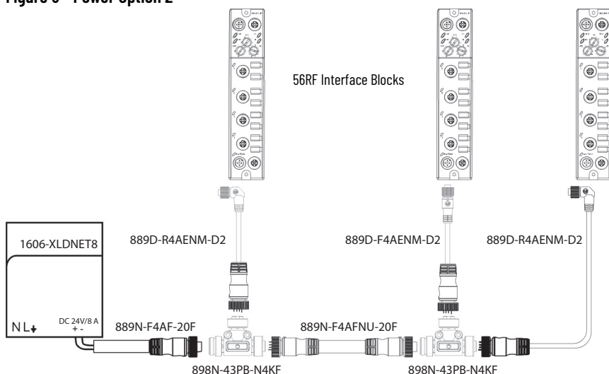
Figure 8 - Power Option 2
