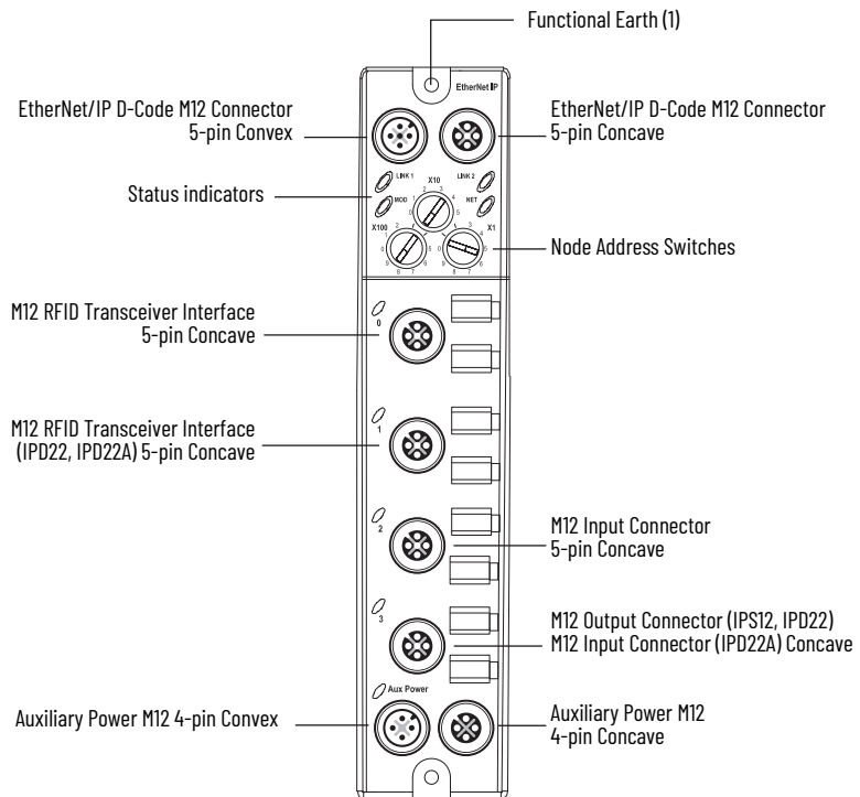
Figure 2 - Connections
