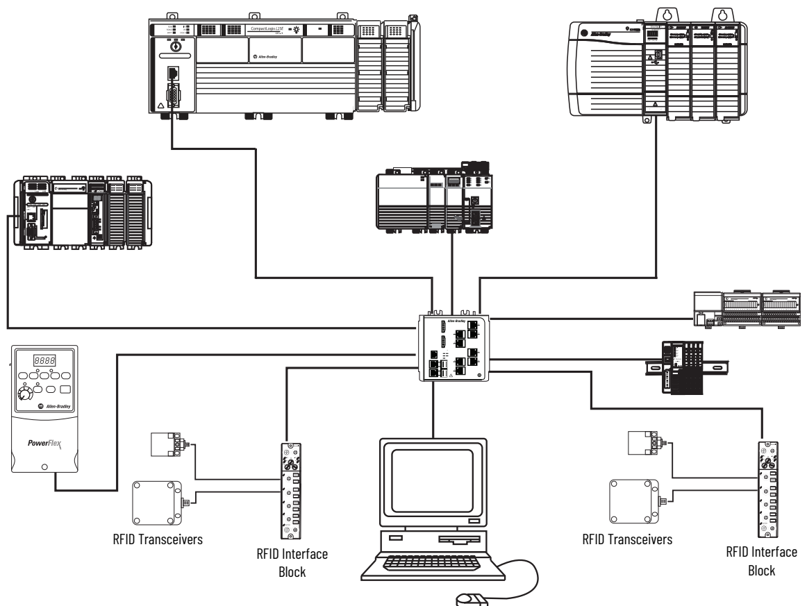
Figure 9 - Star Topology
