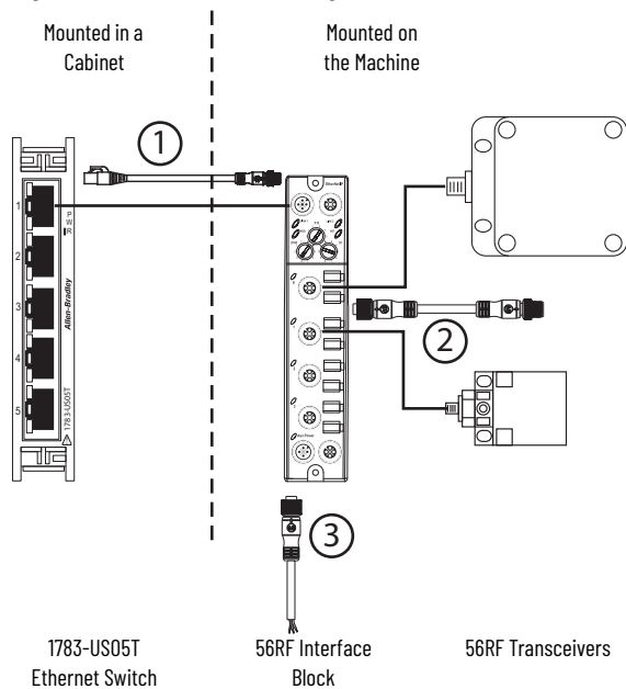
Figure 5 - Transceiver Mounting
