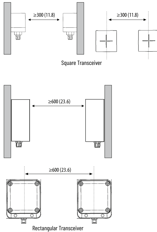
Figure 13 - Spacing Between Transceivers [mm (in.)]
