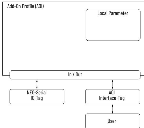
Figure 21 - AOI Interface
