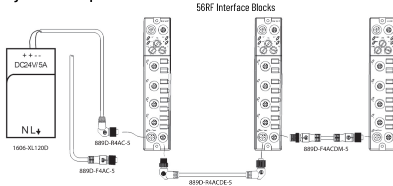
Figure 7 - Power Option 1
