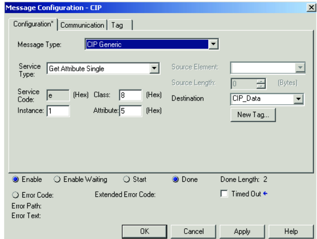
Figure 35 - Obtain Input Filter Off/On Value
