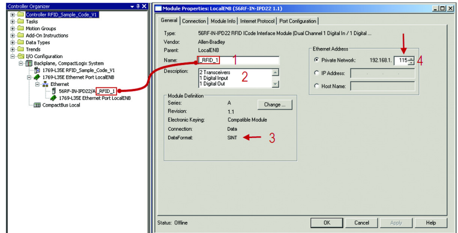
Figure 19 - General Tab
