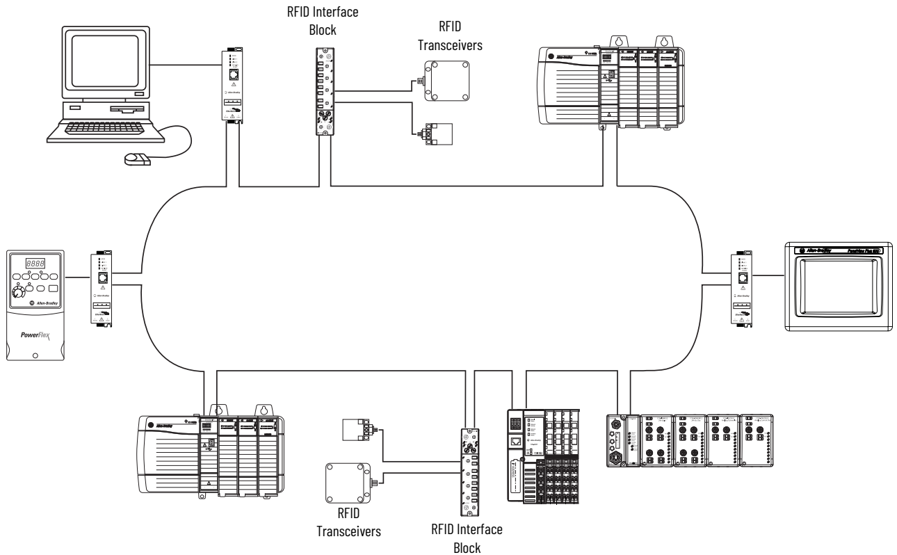
Figure 11 - DLR Topology
