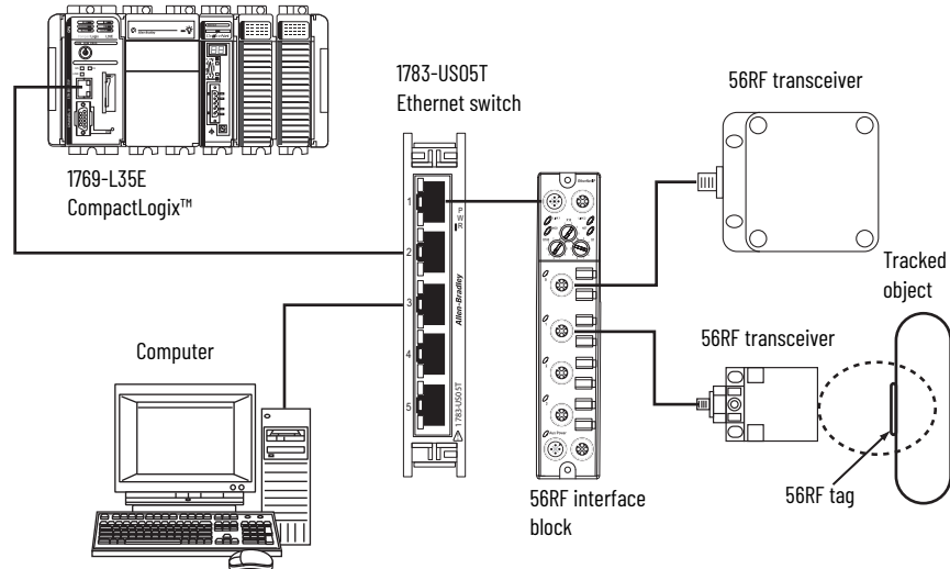
Figure 1 - RFID System
