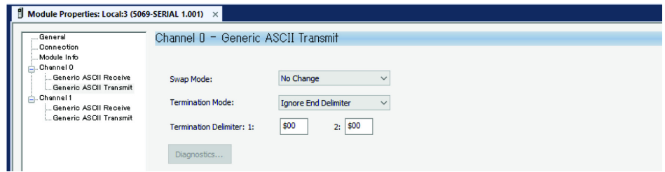
Figure 26 - Module Setting (5/5)
