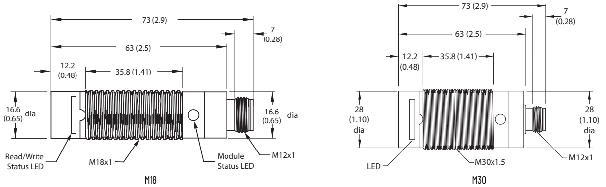
Figure 18 - Cylindrical Transceivers
