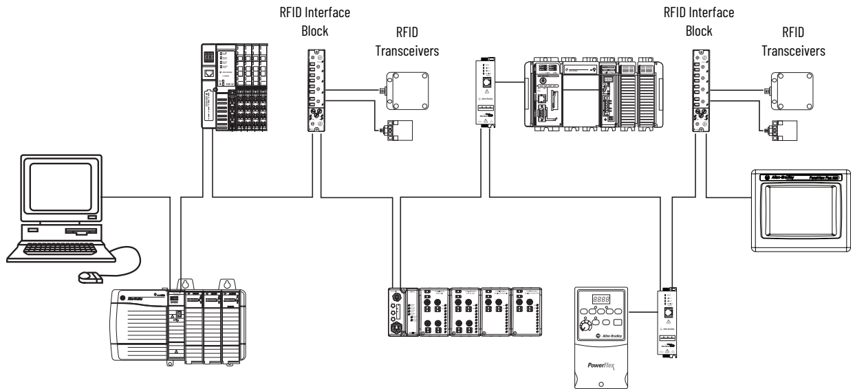
Figure 10 - Linear Topology
