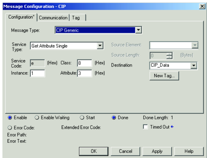
Figure 34 - Obtain Status of Input
