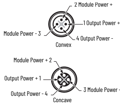
Figure 6 - Pin Connections for the Aux Power Connectors
