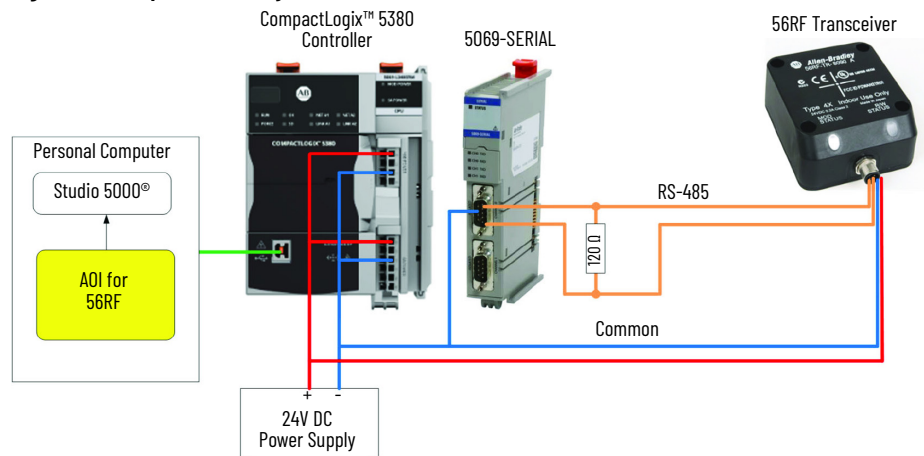
Figure 20 - Proposed 56RF System
