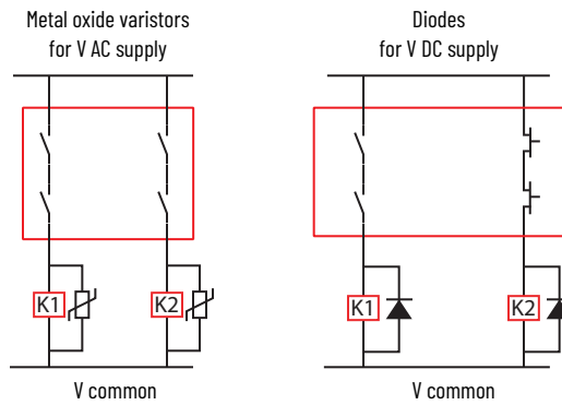
Figure 40 - Surge Protection Examples
