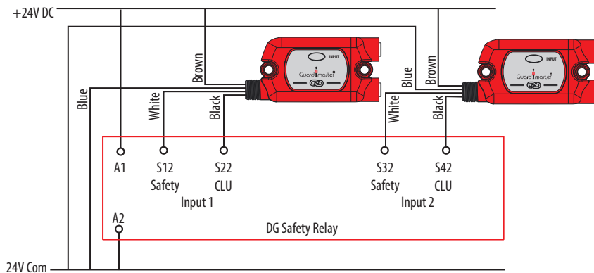
Figure 34 - GuardLink Connections
