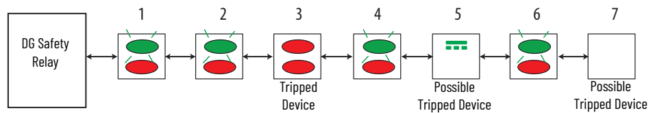
Figure 42 - Tripped Device with Steady Red Status Indicators
