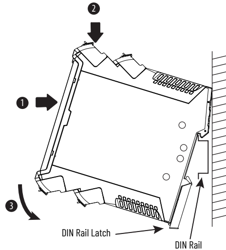
Figure 13 - DIN Rail Mounting
