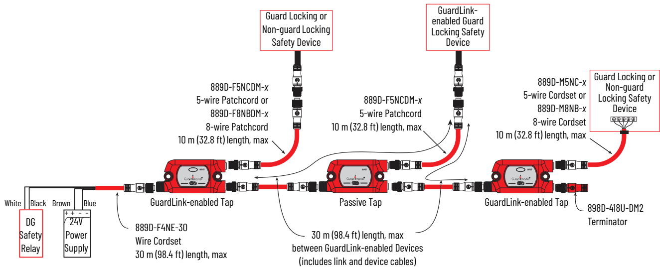
Figure 7 - Example Guard Locking Circuit
