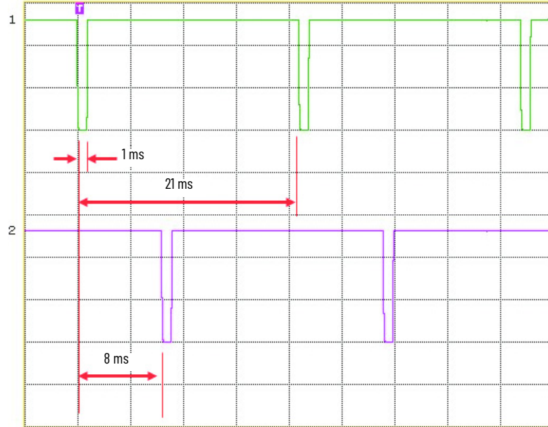
Figure 44 - EMSS Test Pulses
