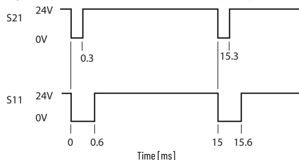
Figure 43 - Pulse Test Sequence for DG Safety Relay
