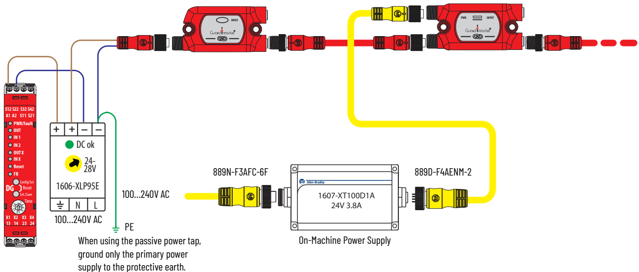
Figure 32 - Multiple Power Supplies on One GuardLink Circuit
