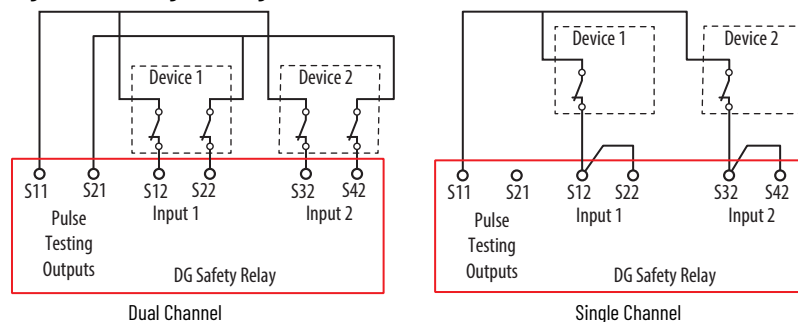
Figure 36 - Wiring to Voltage-free Contacts
