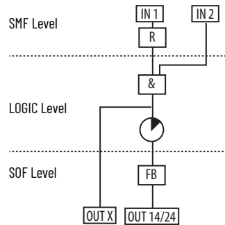
Figure 67 - No SWS, Two Safety Inputs, Monitored Manual Reset Assigned to Input 1, Automatic Reset Assigned to Input 2 Schematic
