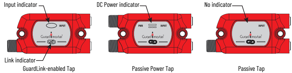
Figure 41 - Tap Indicators
