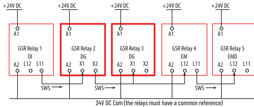
Figure 37 - SWS Connection Example
