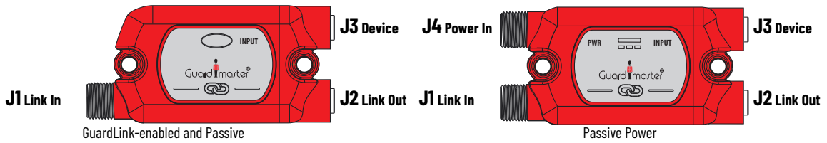
Figure 21 - Tap Connection Identification
