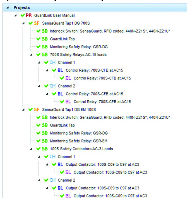
Figure 49 - SISTEMA Project - First Two Safety Functions
