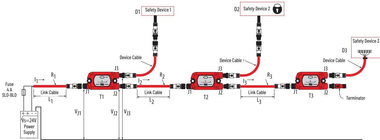
Figure 6 - Tap Connections
