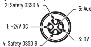
Figure 25 - J3 5-pin OSSD (Female) Connector on 440S-SF5D Tap
