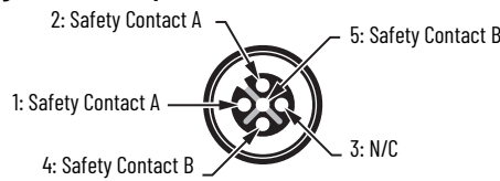
Figure 26 - J3 5-pin EMSS (Female) Connector on 440S-MF5D Tap
