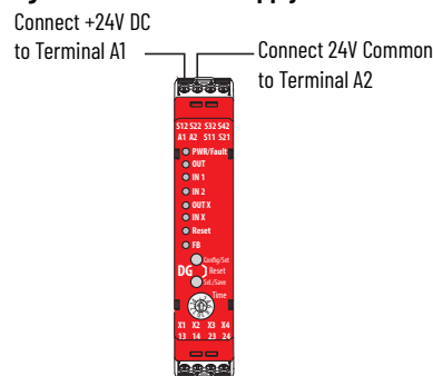
Figure 30 - DG Power Supply Connections
