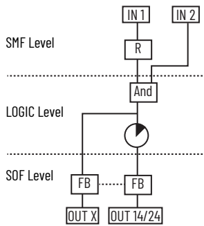
Figure 57 - Two Safety Inputs, First SWS Device, Monitored Manual Reset Assigned to Input 1, Automatic Reset Assigned to Input 2
