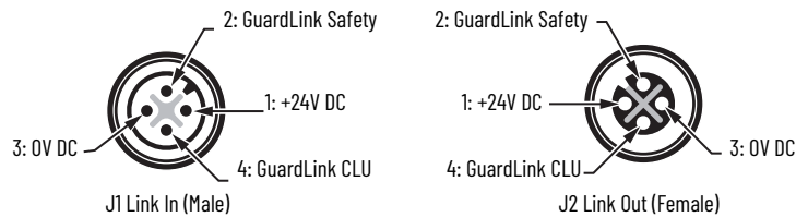
Figure 22 - J1 and J2 Link Connections on All Taps
