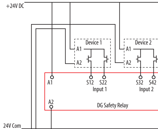
Figure 35 - Wiring to Devices with OSSD Outputs
