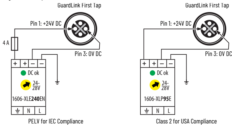
Figure 31 - Tap Power Connections
