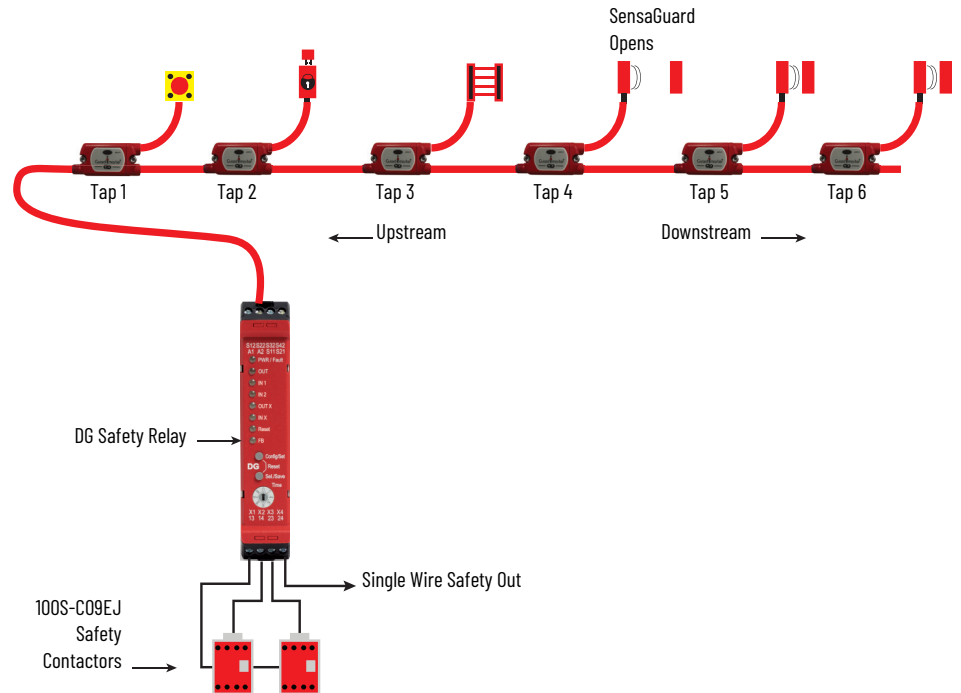
Figure 10 - Response Time Example Calculation
