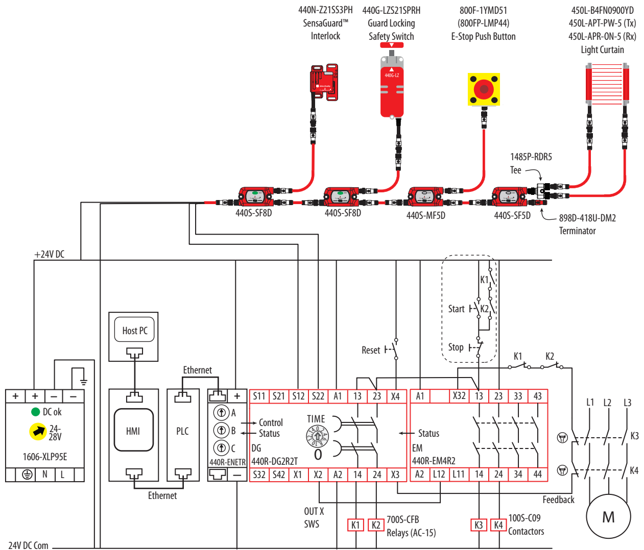
Figure 47 - Example Circuit for Safety System Calculation
