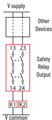
Figure 39 - Output Connections of the DG Safety Relay
