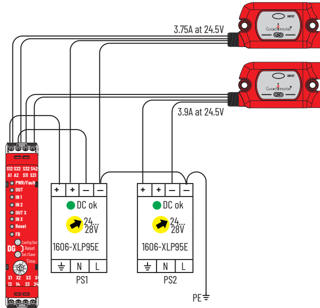
Figure 33 - Multiple Power Supplies on Two GuardLink Circuits
