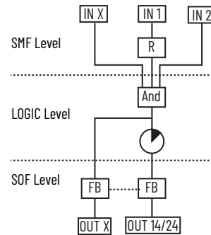
Figure 52 - Two Safety Inputs, Middle SWS, Monitored Manual Reset Assigned to Input 1, Automatic Reset Assigned to Input 2
