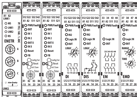
Figure 46 - 440R-ENETR Interface Arrangement
