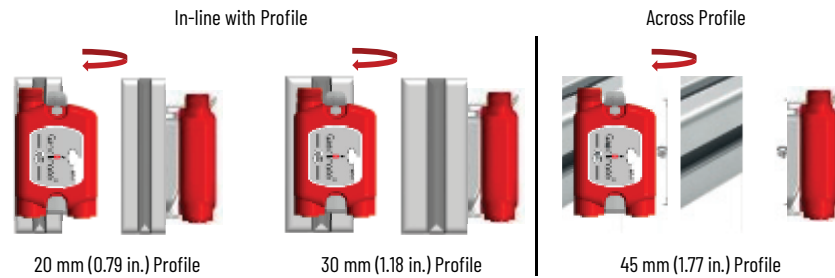
Figure 19 - Mounting Options with Quick-release Bracket
