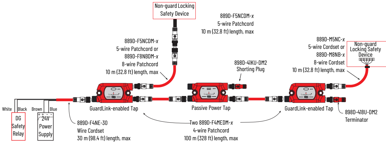
Figure 8 - Example of a Non-guard Locking Circuit
