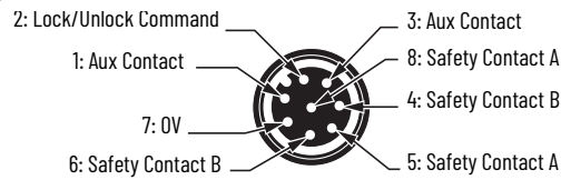
Figure 24 - J3 8-Pin EMSS (Female) Connector on 440S-MF8D and 440S-MLF8D Taps
