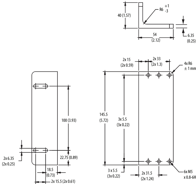
Figure 6 - Switch Mounting Bracket (440G-LZAM2) [mm (in.)]
