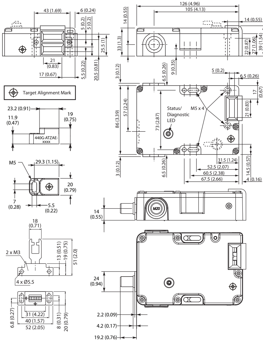
Figure 8 - Guard Locking Switch [mm (in.)]
