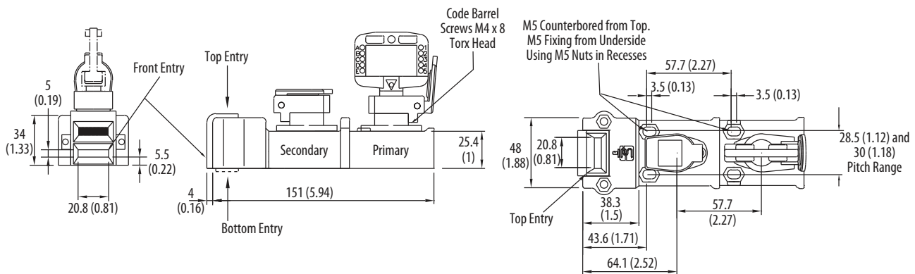
Figure 110 - Actuators [mm (in.)]
