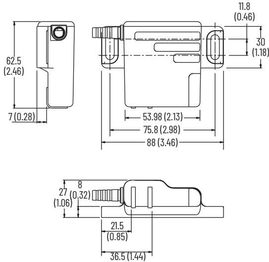
Figure 34 - Integrated Latch [ mm (in.) ]
