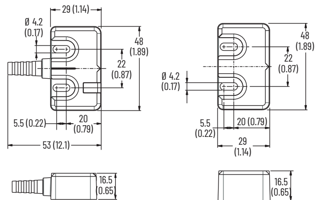
Figure 36 - MC2 [mm (in.)]
