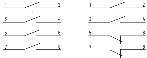
Figure 77 - Diagrams Shown with Key Free
