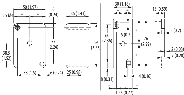
Figure 38 - Interlock Switch Dimensions [mm (in.)]
