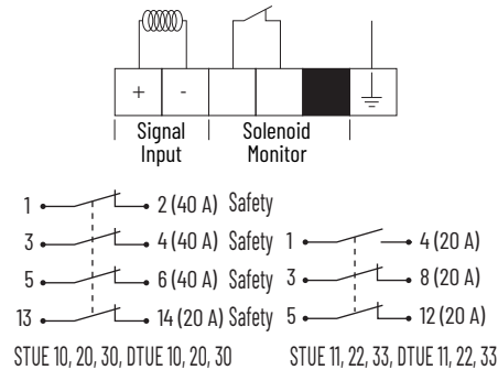
Figure 82 - Wiring (Shown with Power On)
