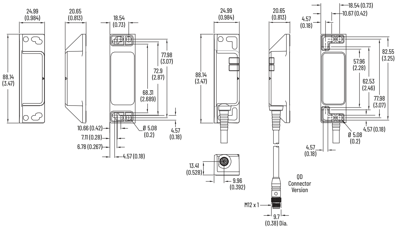
Figure 33 - Large Rectangular Flat Pack [mm (in.)]
