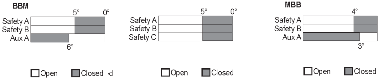
Figure 26 - Contact Action
