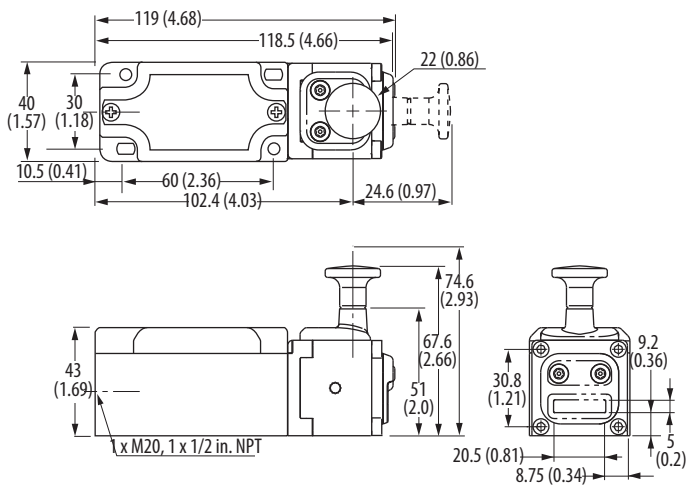
Figure 57 - MT-GD2 Latch Release [mm (in.)]
