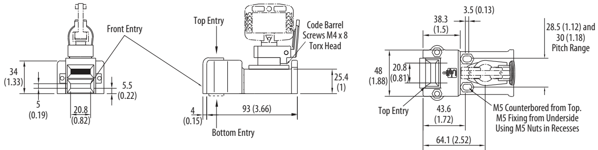
Figure 109 - Dual Key Slamlock [mm (in.)]
