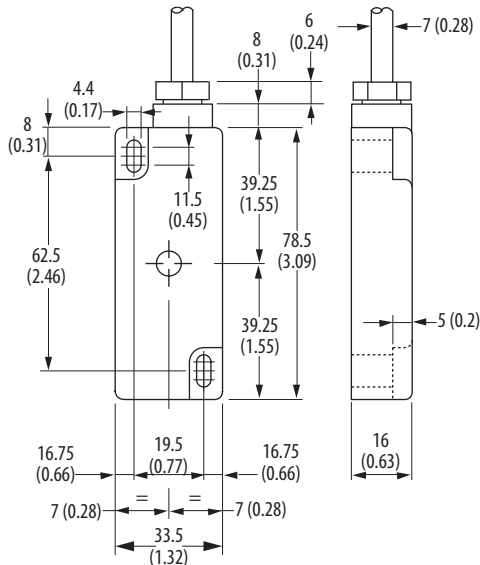
Figure 43 - Actuator [mm (in.)]
