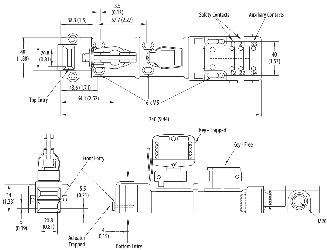
Figure 112 - Electrical Dual Key Slamlock [mm (in.)]
