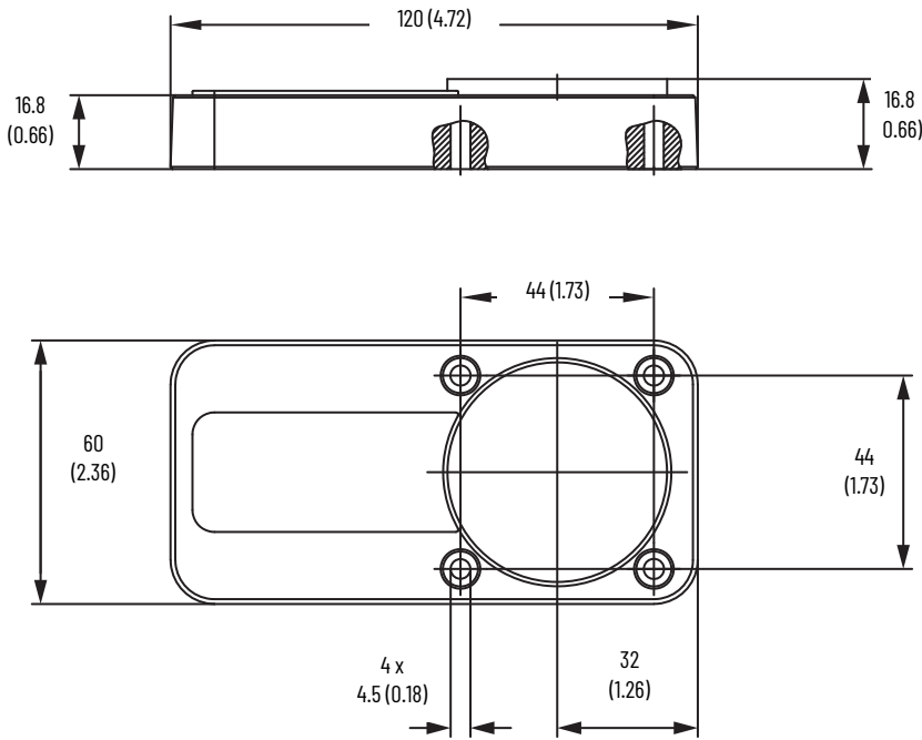
Figure 30 - Actuator [mm (in.)]
