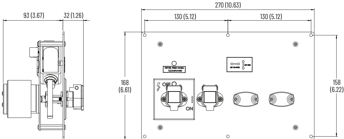
Figure 79 - Multi-key [mm (in.)]
