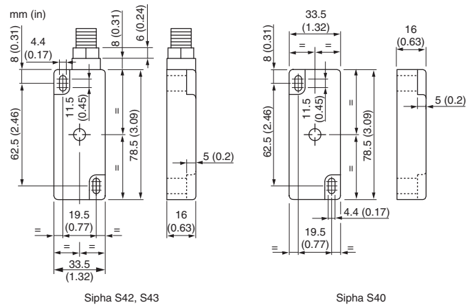
Figure 49 - Siphon S4 [mm (in.)]
