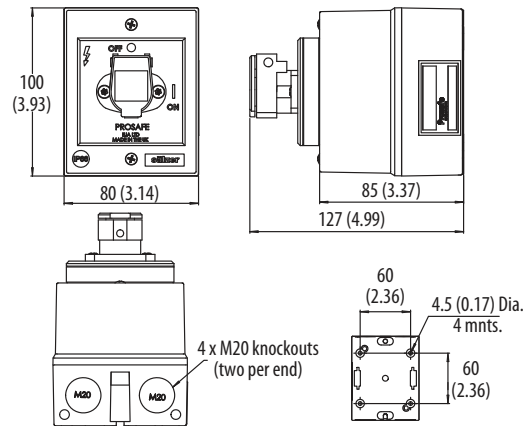
Figure 67 - RKSE12 and RKSE13 [mm (in.)]
