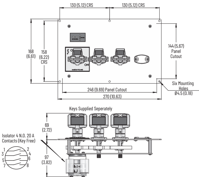
Figure 64 - MRXE10 and MRXE11 [mm (in.)]
