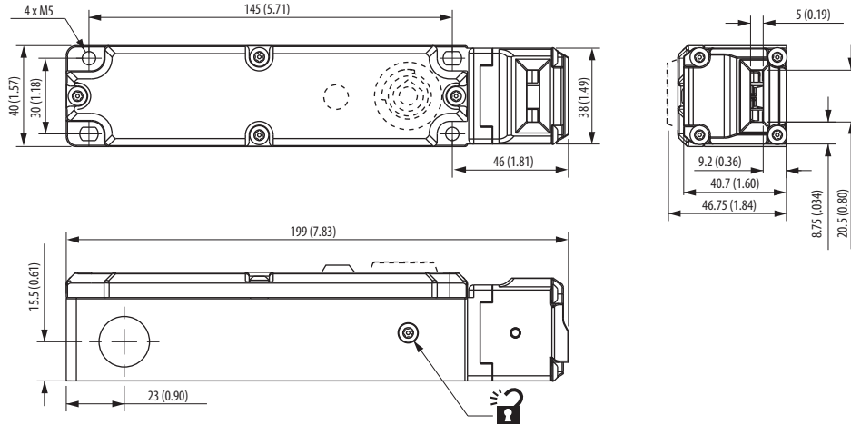
Figure 11 - Guard Locking Switch [mm (in.)]
