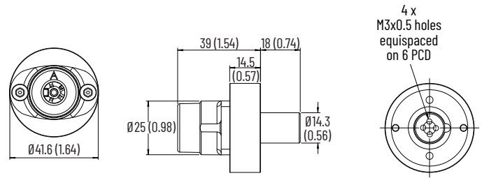
Figure 118 - 440T-MSGAU23x [mm (in.)]
