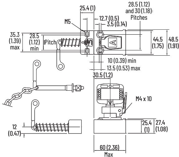
Figure 103 - Mechanical, Dual Key, Lever Actuator [mm (in.)]
