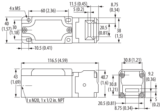
Figure 57 - MT-GD2 Latch Release [mm (in.)]
