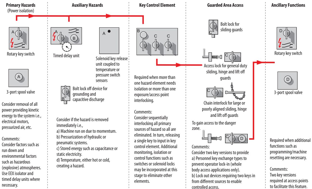
Figure 58 - Plant and Machinery Interlocking
