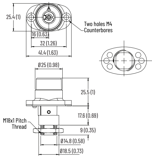
Figure 116 - 440T-MSGAU20x [mm (in.)]
