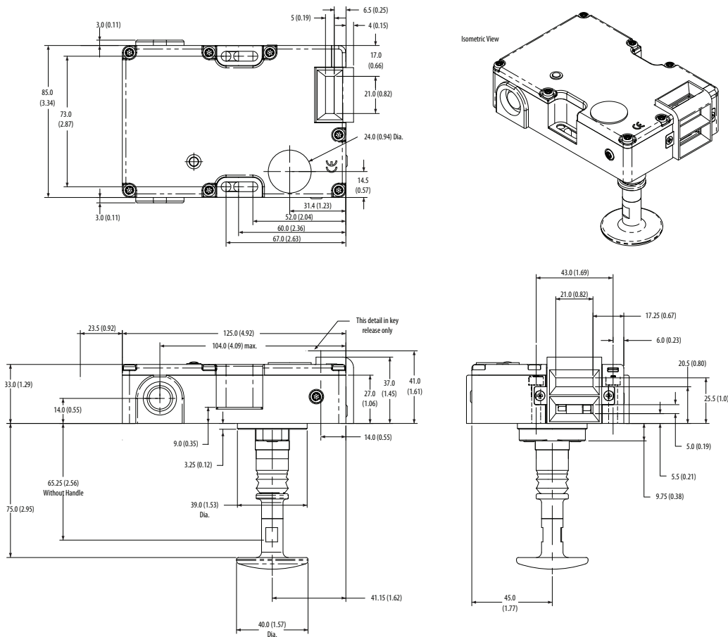
Figure 10 - TLS-GD2 Escape Release [mm (in.)]
