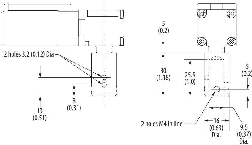
Figure 19 - Hollow Shaft
