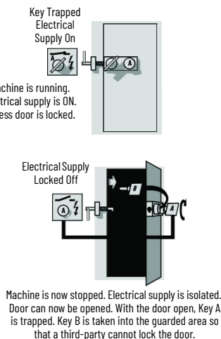
Figure 61 - Full Body Access
