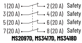
Figure 81 - Contacts
