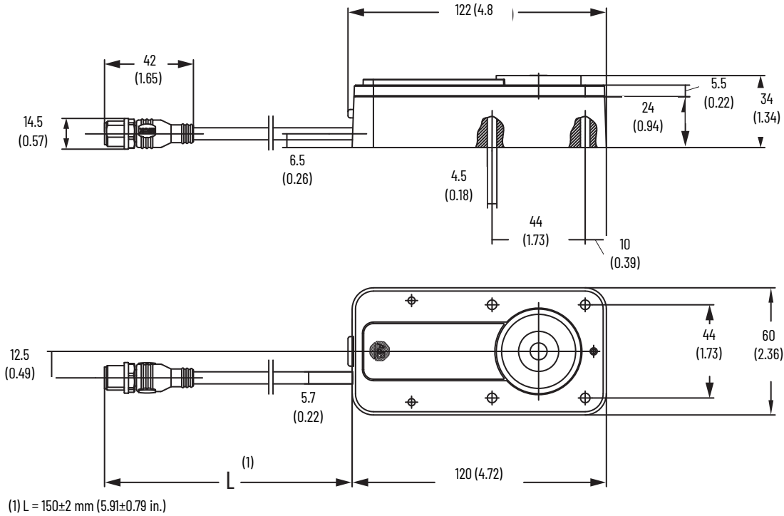
Figure 31 - Sensor [mm (in.)]
