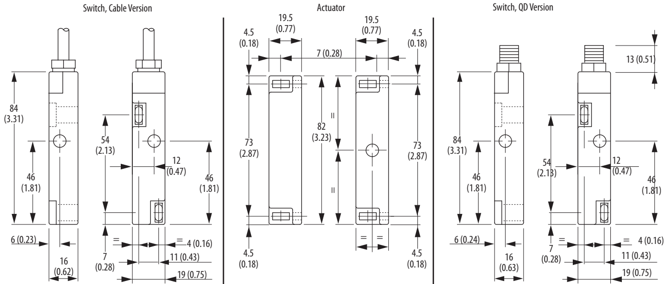
Figure 41 - FRS 13 and 14 [mm (in.)]
