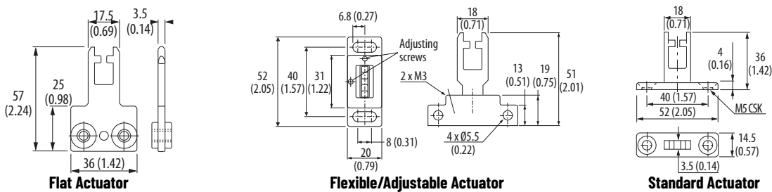
Figure 110 - Actuators [mm (in.)]
