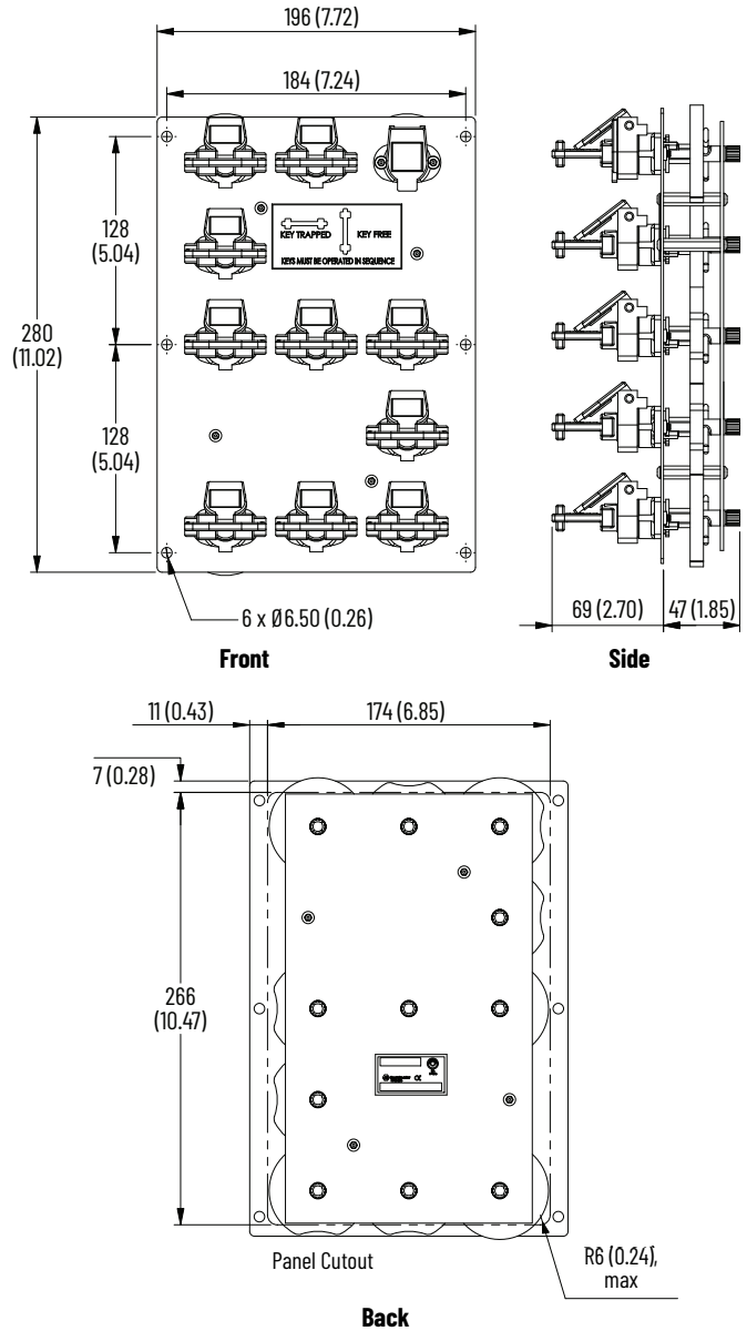
Figure 86 - 7-...11-way Units [mm (in.)]
