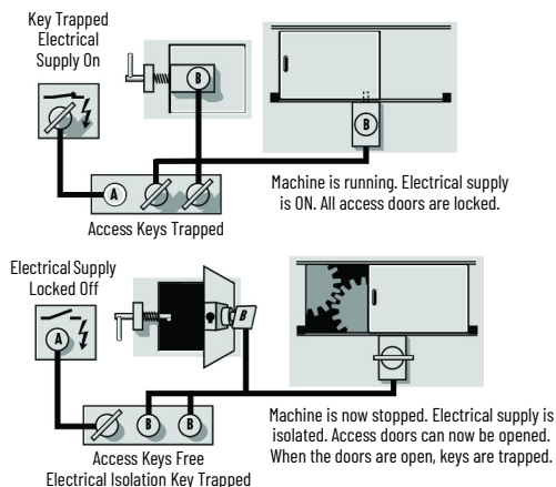
Figure 60 - Part Body Access
