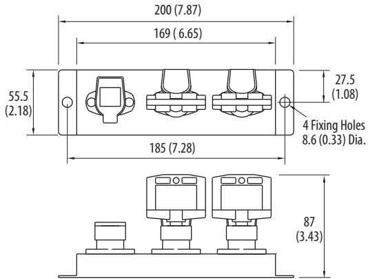
Figure 85 - 4-, 5-, or 6-way Key Exchange Unit [mm (in.)]
