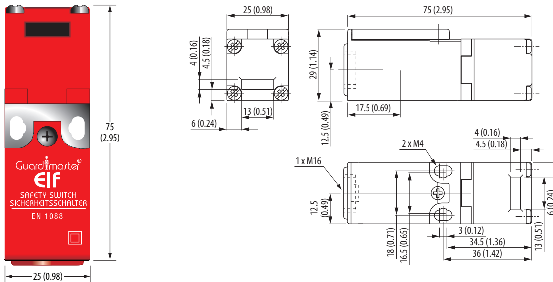
Figure 50 - Interlock Switch Dimensions [mm (in.)]
