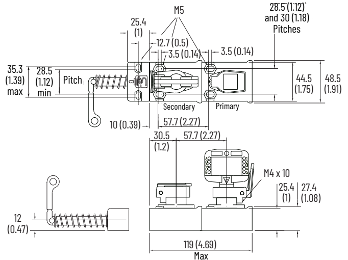
Figure 105 - Electrical, Dual Key, Chain Actuator [mm (in.)]
