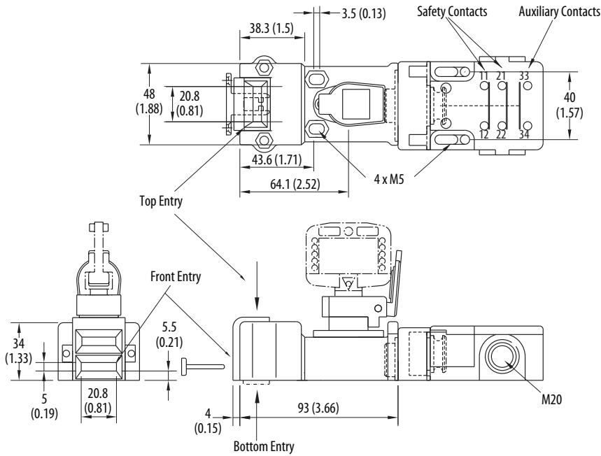
Figure 112 - Electrical Dual Key Slamlock [mm (in.)]
