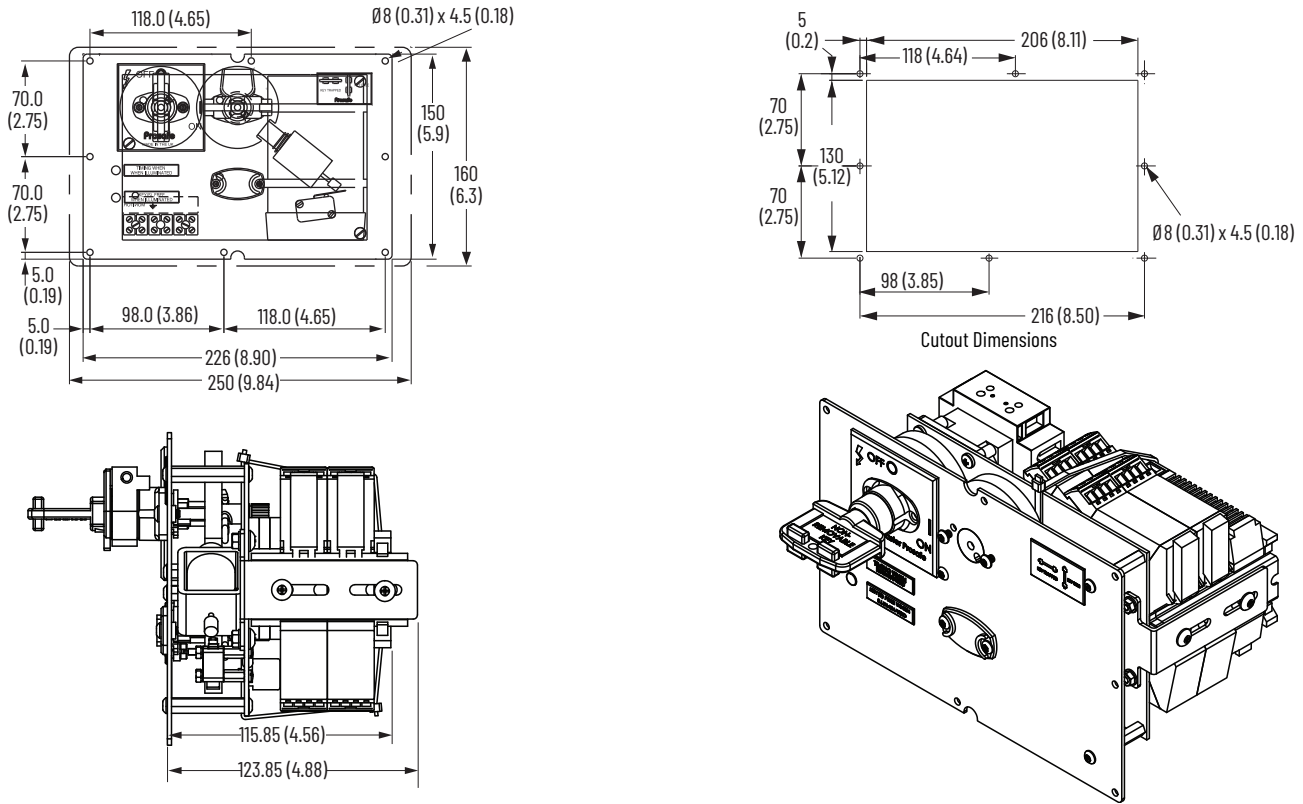
Figure 83 - Timed-delay Unit Dimensions [mm (in.)]
