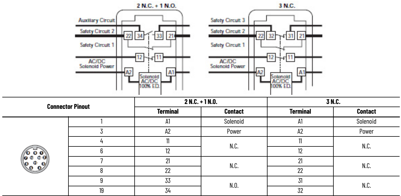
Figure 16 - Contact Action
