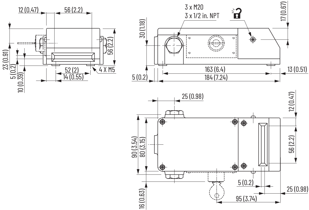
Figure 12 - Guard Locking Switch Dimensions [mm (in.)]
