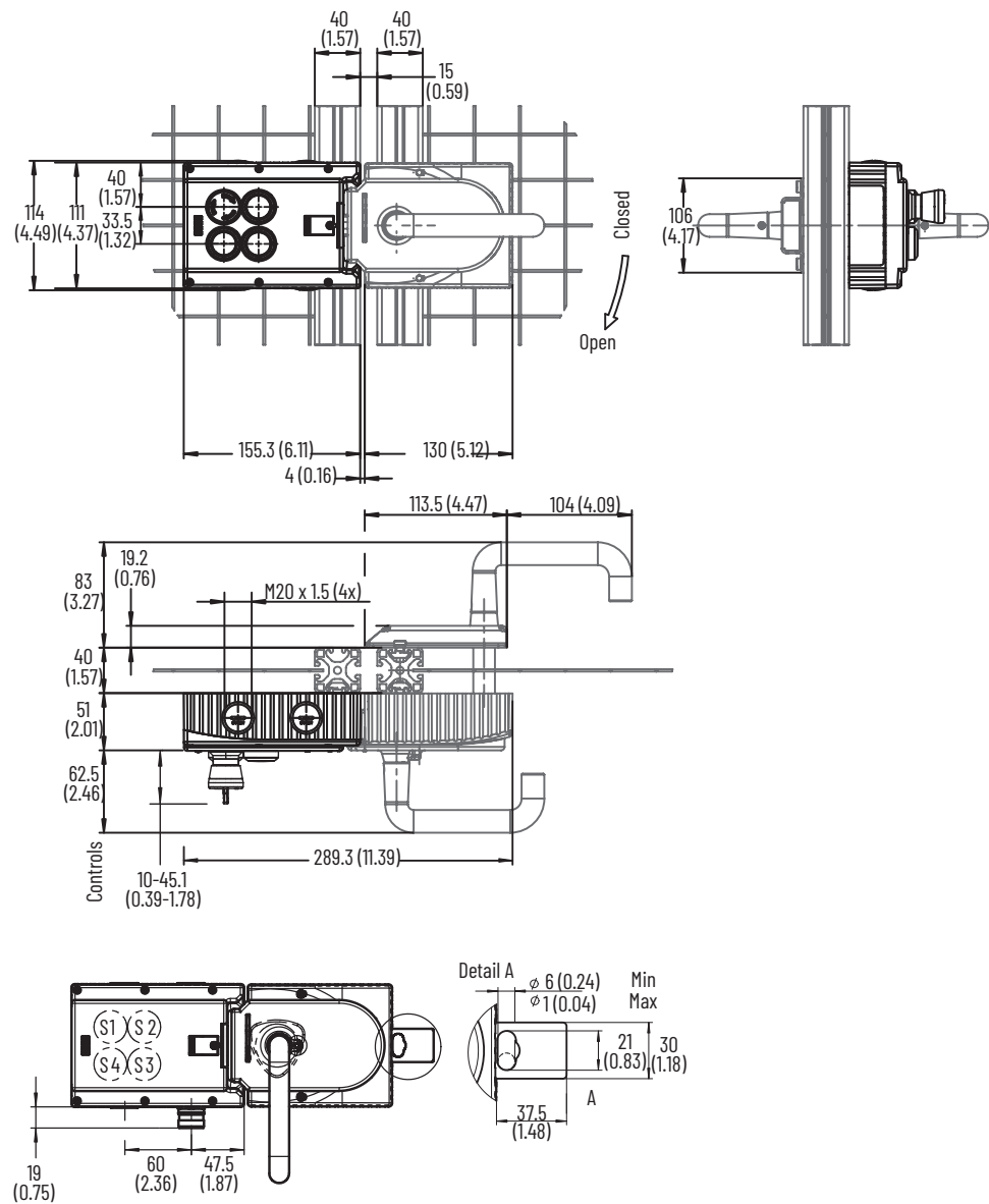
Figure 120 - 442G-MAB [mm (in.)]
