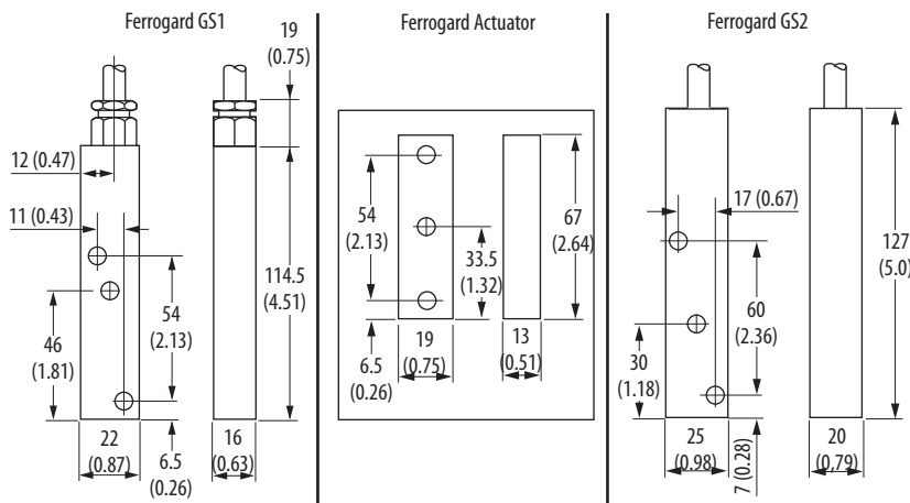
Figure 44 - Interlock Switch Dimensions [mm (in.)]
