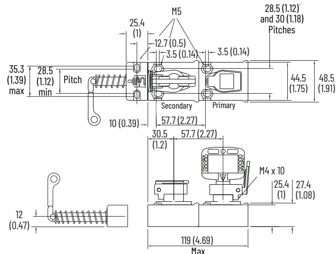
Figure 103 - Mechanical, Dual Key, Lever Actuator [mm (in.)]
