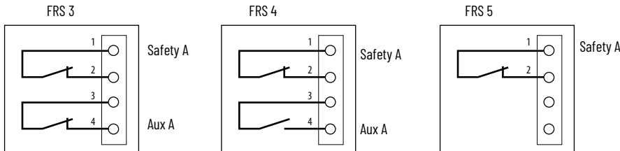
Figure 39 - Interlock Switch Wiring
