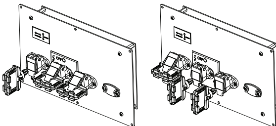
Figure 76 - Multi-key (One Key In/Two Keys Out)
