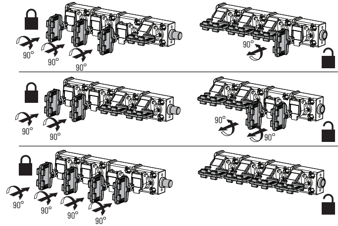
Figure 93 - Quad Key
