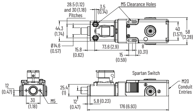
Figure 100 - Prosafe Bolt Lock Solenoid Locked with Electrical Isolation - One Key [mm (in.)]
