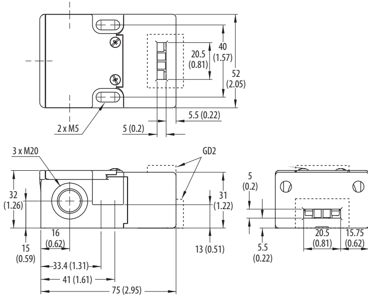
Figure 53 - Interlock Switch Dimensions [mm (in.)]
