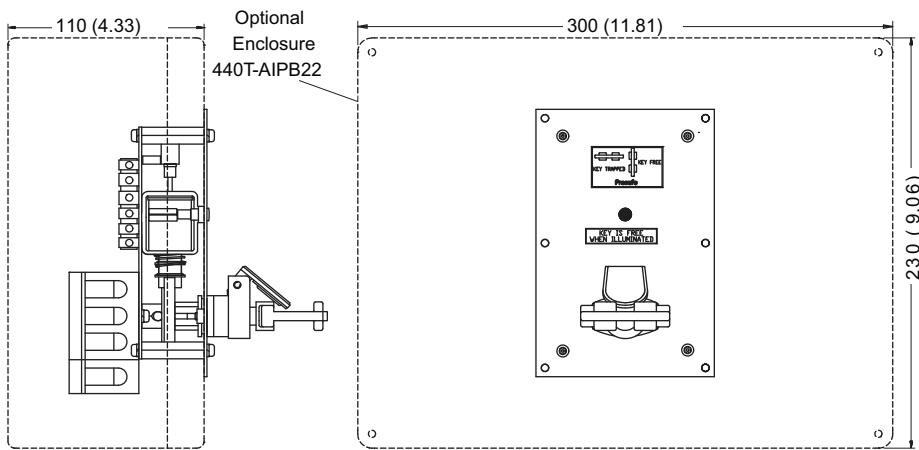
Figure 79 - Multi-key [mm (in.)]
