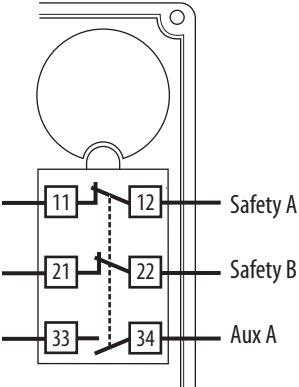
Figure 29 - Contact Configuration 2 N.C. and 1 N.O.
