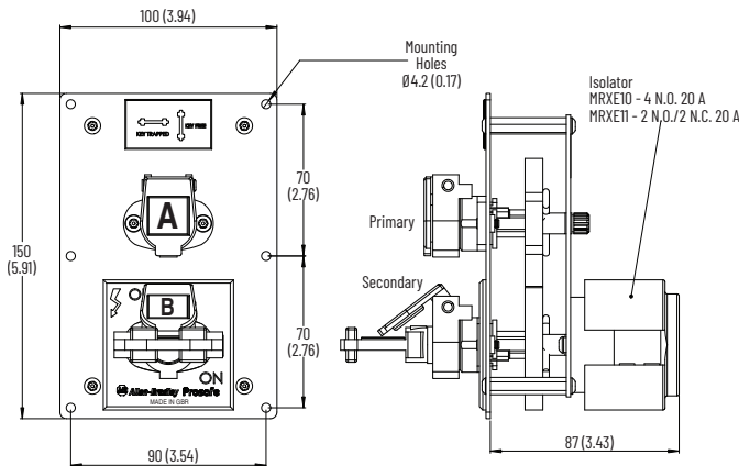
Figure 64 - MRXE10 and MRXE11 [mm (in.)]
