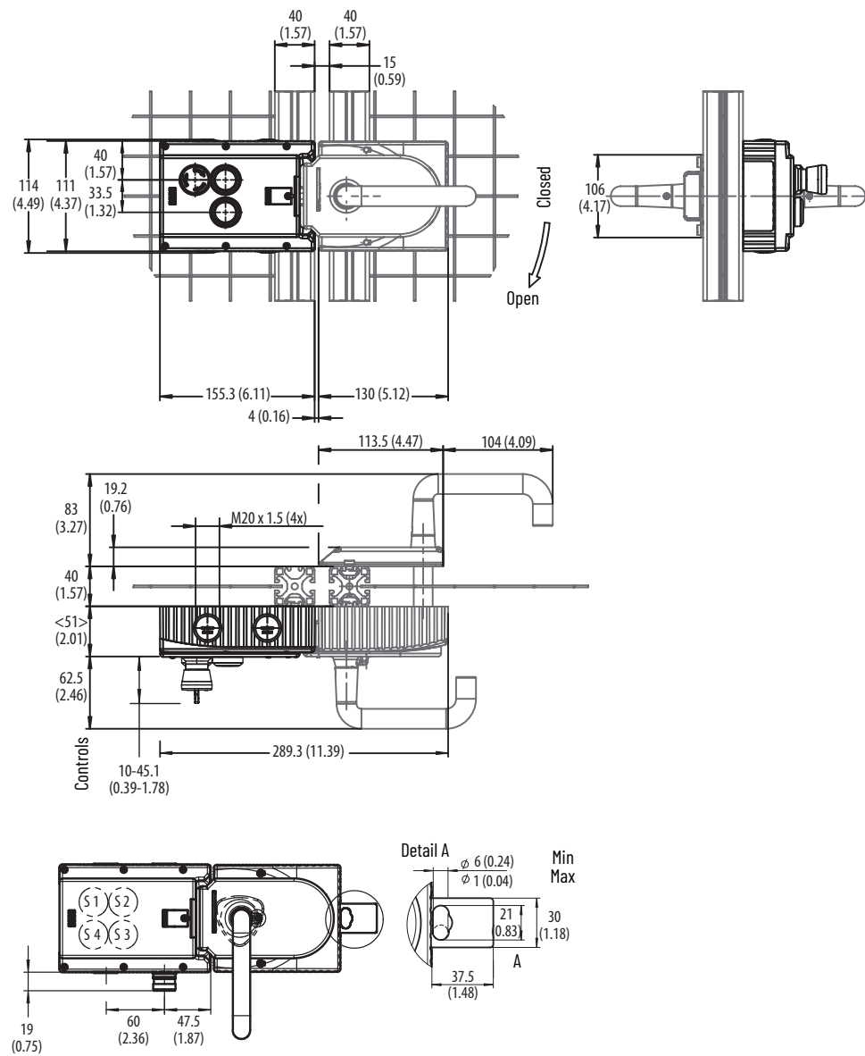
Figure 119 - 442G-MAB [mm (in.)]
