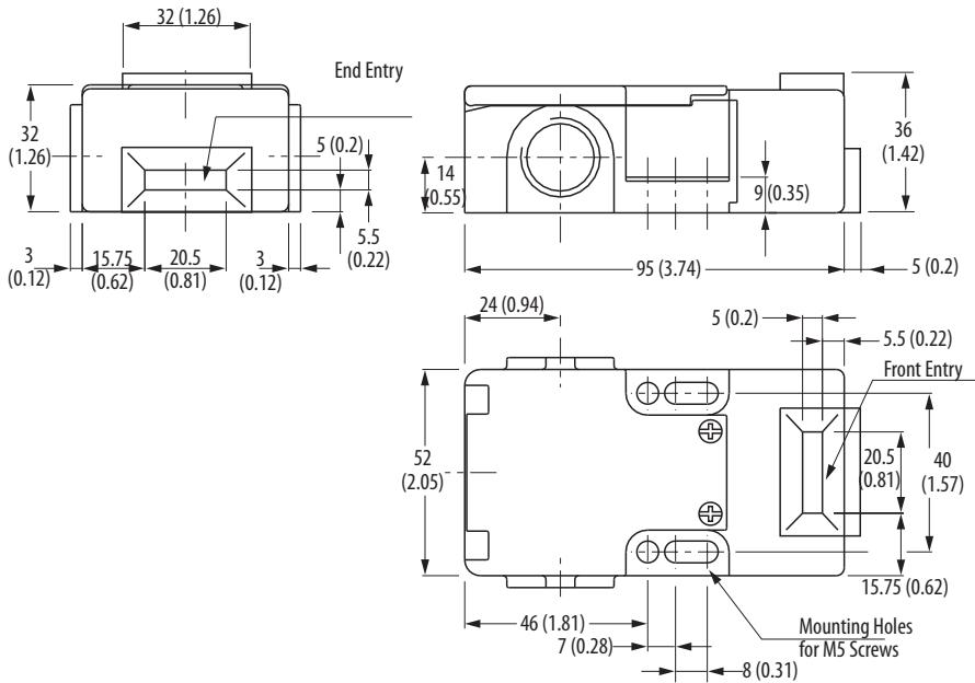
Figure 55 - GD2 Model [mm (in.)]
