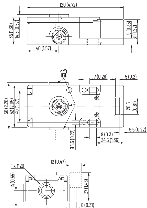
Figure 15 - Guard Locking Switch [mm (in.)]
