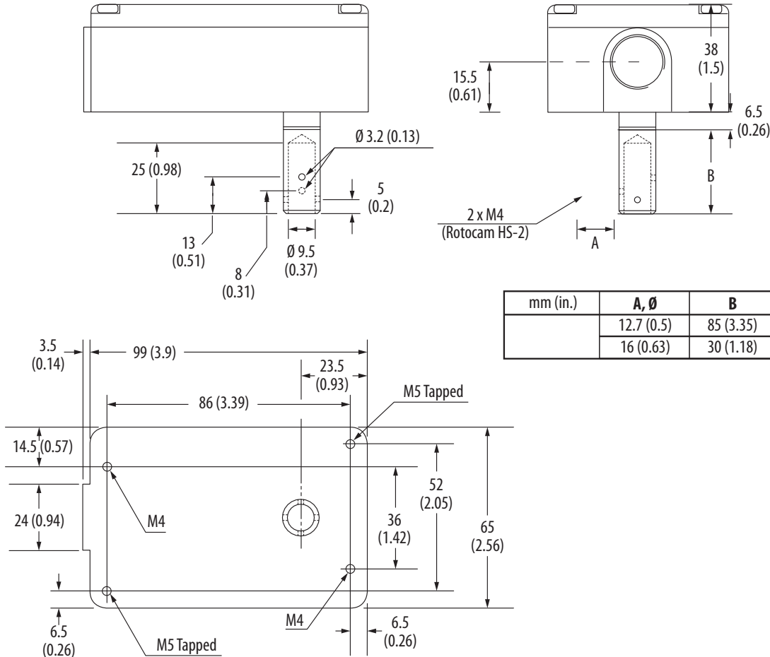
Figure 28 - Hinge Interlock Switch [mm (in.)]
