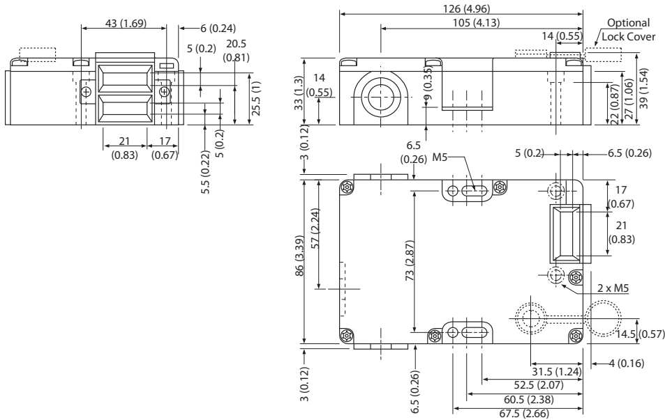
Figure 9 - Guard Locking Switch Dimensions [mm (in.)]
