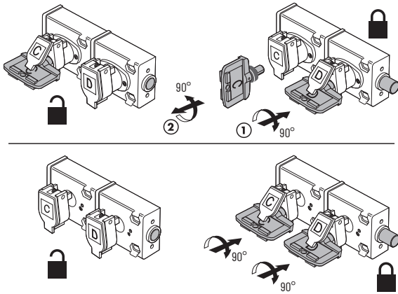
Figure 91 - Dual Key
