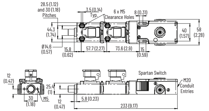
Figure 101 - Prosafe Bolt Lock Solenoid Locked with Electrical Isolation - Two Keys [mm (in.)]
