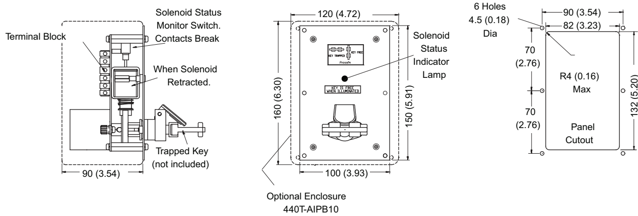
Figure 78 - Single Key [mm (in.)]
