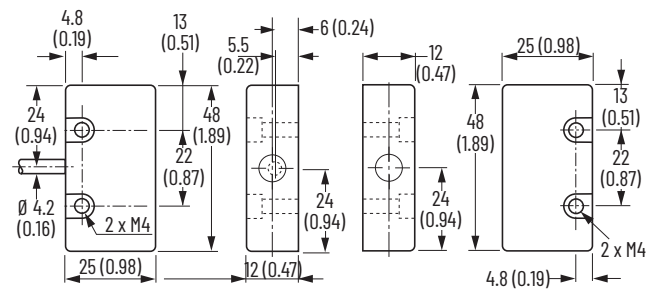
Figure 36 - MC2 [mm (in.)]
