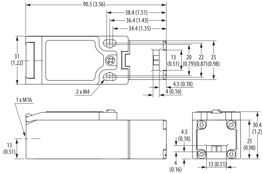
Figure 51 - Interlock Switch Dimensions [mm (in.)]
