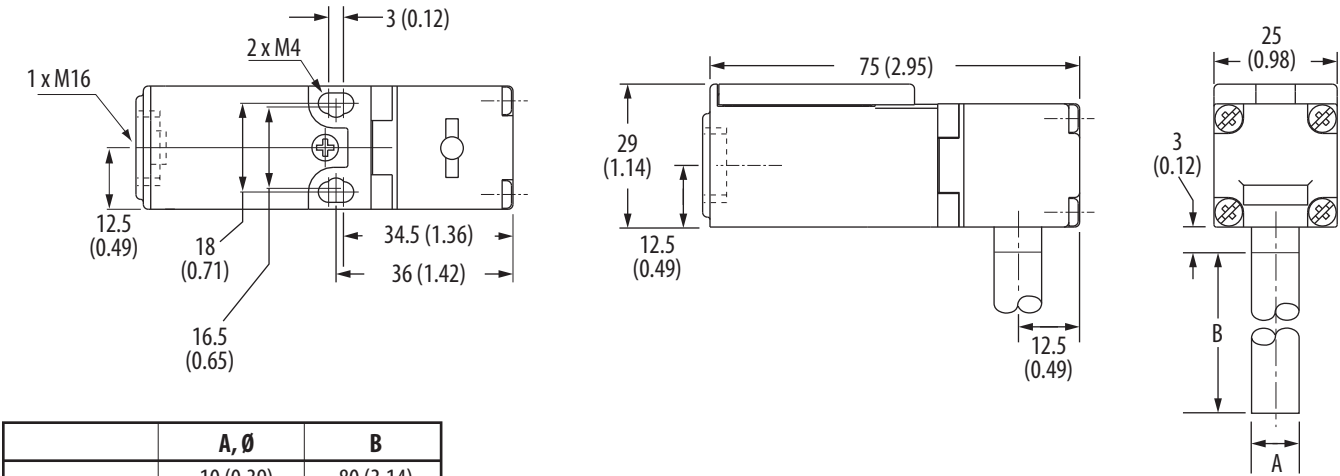
Figure 18 - Hinge Interlock Switch Dimensions [mm (in.)]
