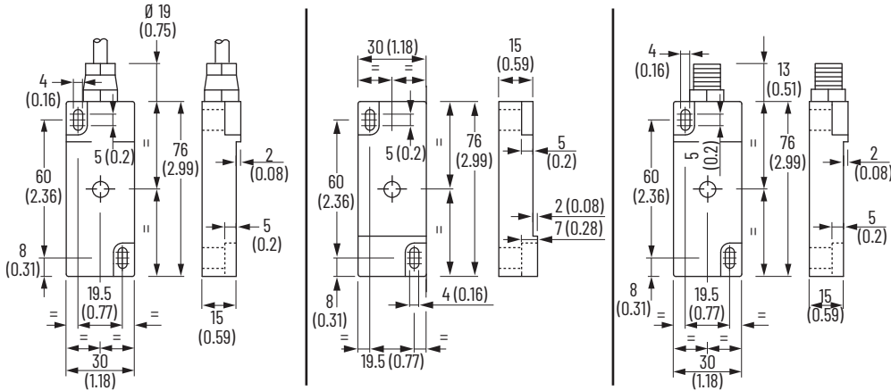
Figure 37 - Interlock Switch Dimensions [mm (in.)]
