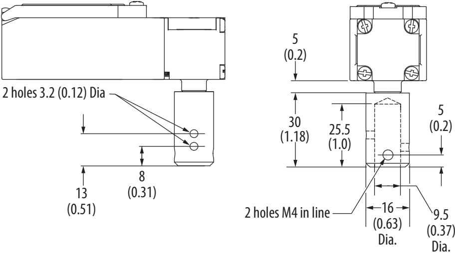
Figure 24 - Hollow Shaft
