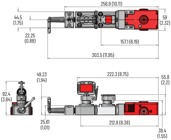
Figure 107 - Solenoid, Dual Key, Lever Actuator [mm (in.)]
