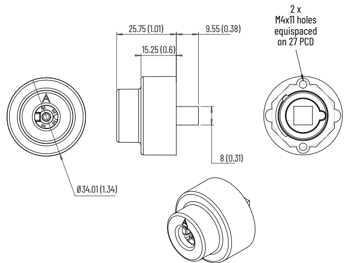
Figure 118 - 440T-MSGAU23x [mm (in.)]
