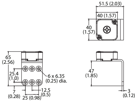
Figure 6 - Switch Mounting Bracket (440G-LZAM2) [mm (in.)]
