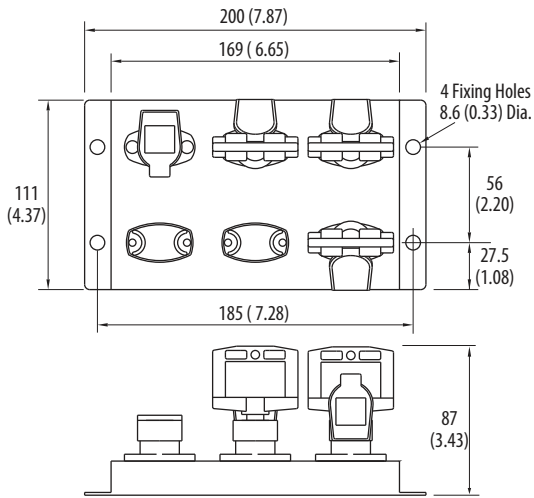
Figure 85 - 4-, 5-, or 6-way Key Exchange Unit [mm (in.)]
