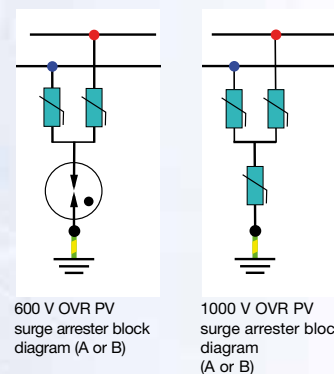
OVR PV surge arrester (A or B)
