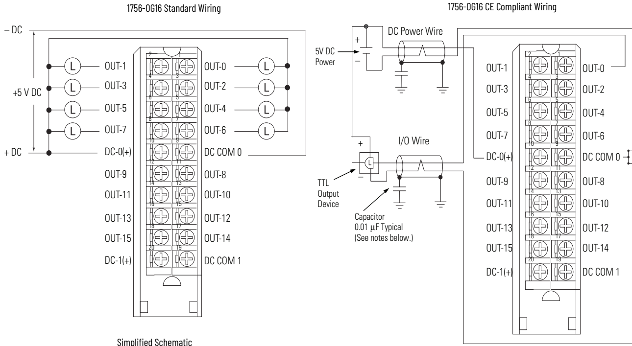
Simplified Schematic
