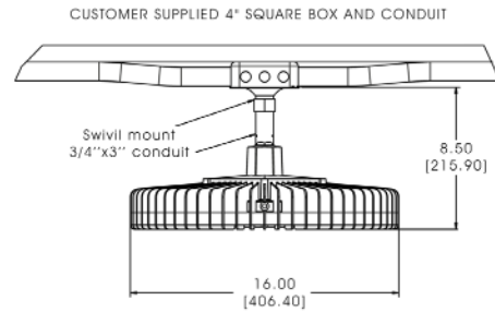
HBXCU - Ceiling Mount
