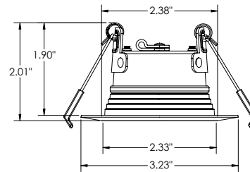
2 1/2" CEILING CUTOUT
